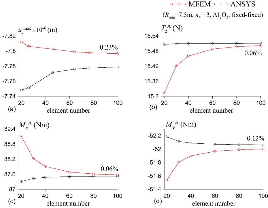
Fig.4. The convergence analysis for the static response of the AFG elliptical beam ( \text{Al}-\text{Al}_2\text{O}_3 ) having fixed-fixed BC
