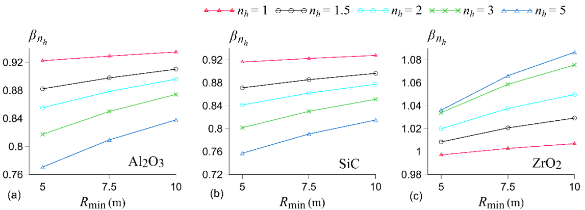
Fig. 5. The effect of the non-homogeneity index on the fundamental natural frequencies of AFG elliptical beam having fixed-fixed BC, \beta_{n_h=i} = f_{n_h=i} / f_{n_h=0.5} where ( i = 1, 1.5, 2, 3 , and 5).
